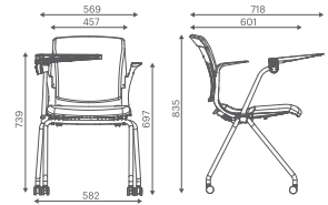
4 Legged Nesting 4-M8PL-0000-M054-M384-A
