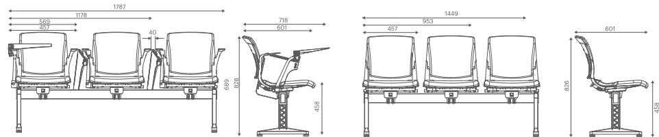
4 Legged With Tray 4-M8PL-0000-M043-M374-A
